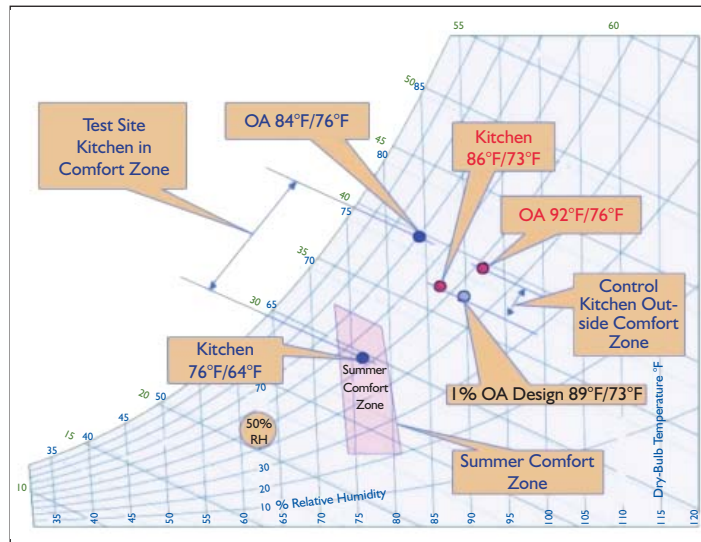
Figure 3: Enthalpy comparison.
